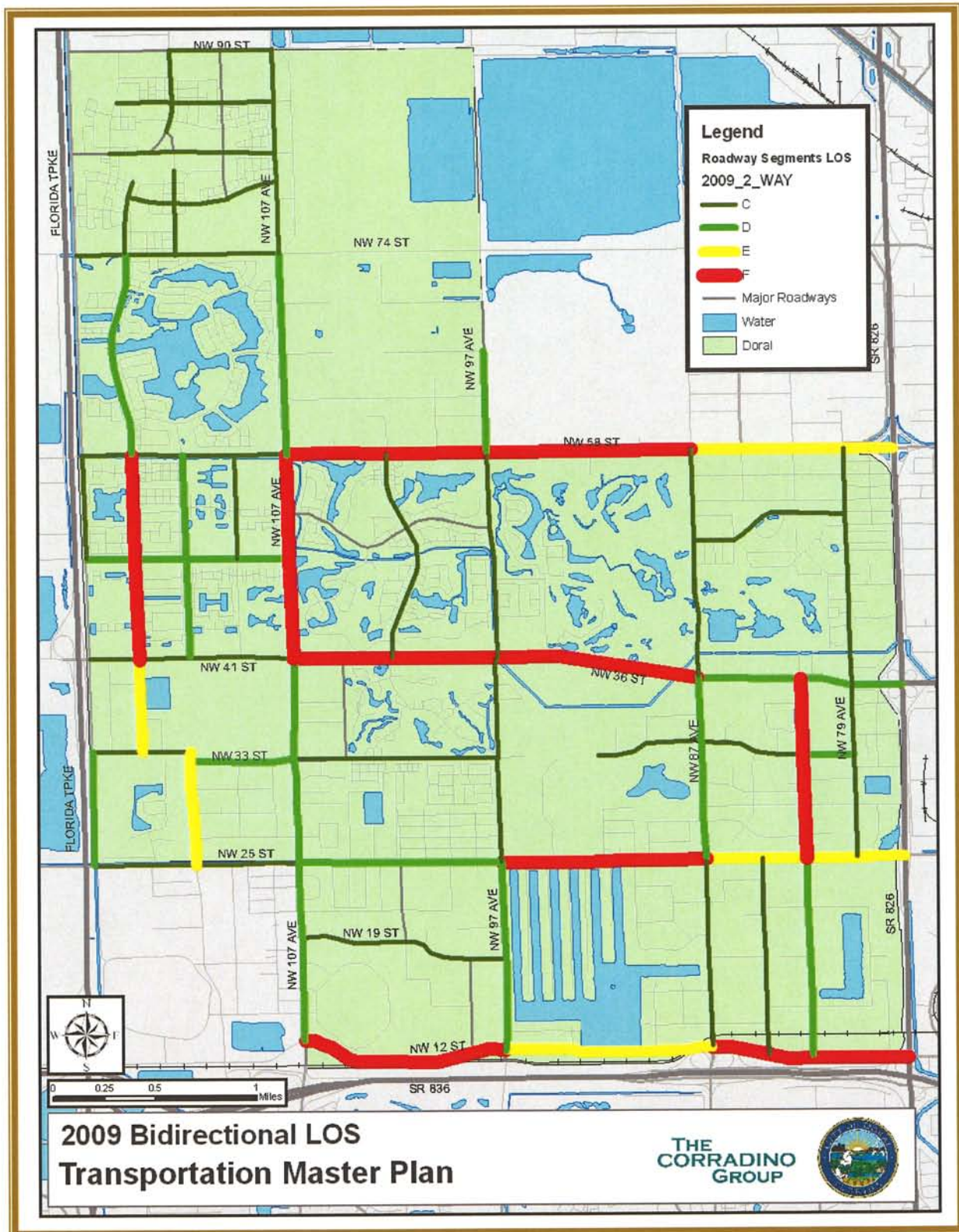
Figure 33 – 2009 Bi-directional Level-of-Service
